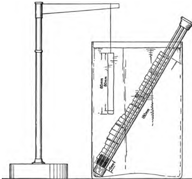
FIG. 6.—Demonstration of the swelling of sections of plates of agar 4 parts, opuntia mucilage 4 parts, gelatin 1 part, bean protein 1 part, in thickness with but little increase in length, due to the manner in which the moist colloid was held while drying.
